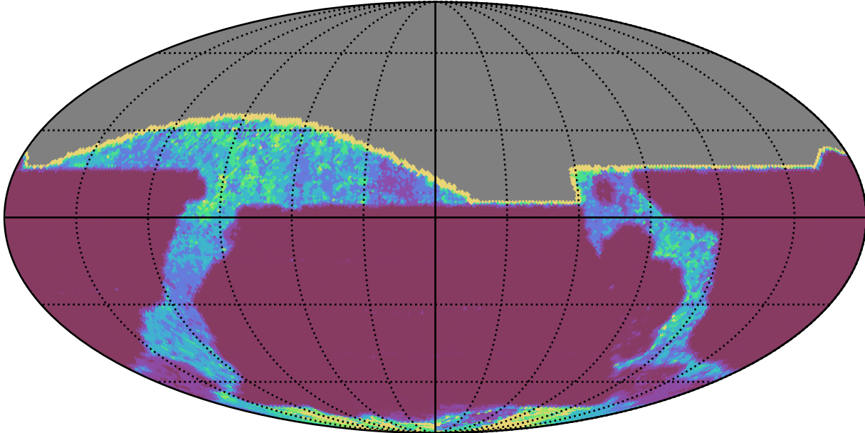
roll_pause_mjdp120_v3.4_10yrs All sky all bands: 20thPercentile Inter-Night Gap
