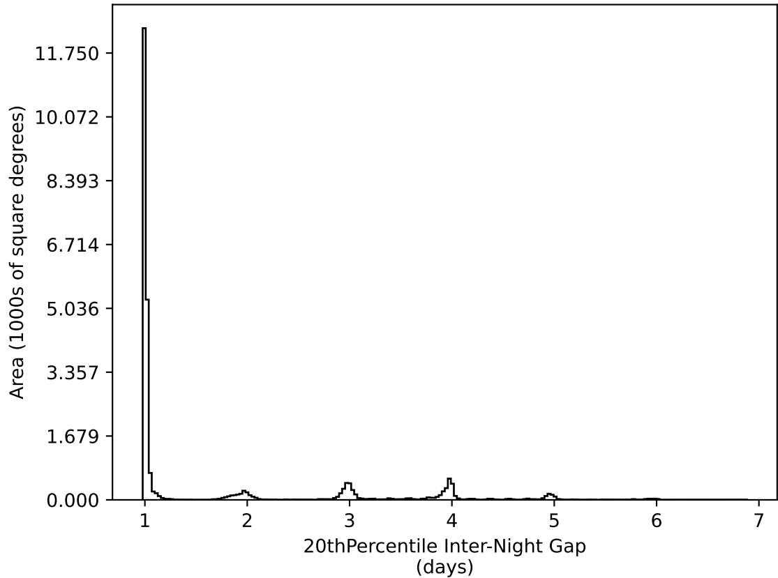
roll_pause_mjdp120_v3.4_10yrs All sky all bands: 20thPercentile Inter-Night Gap
