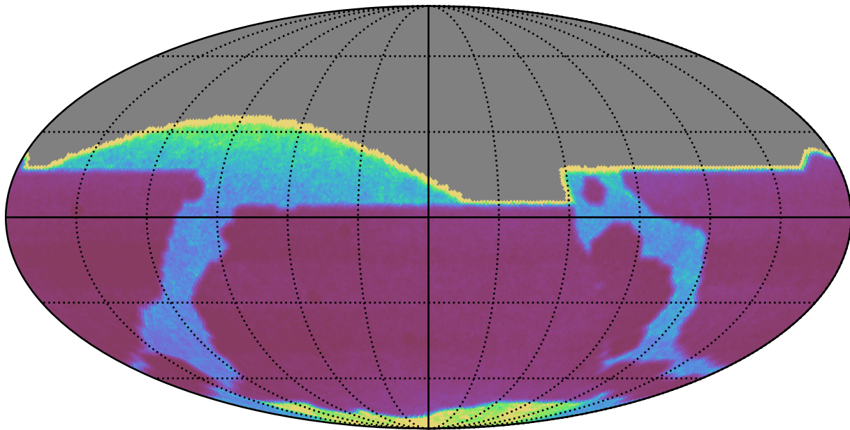
roll_pause_mjdp120_v3.4_10yrs : properMotion
