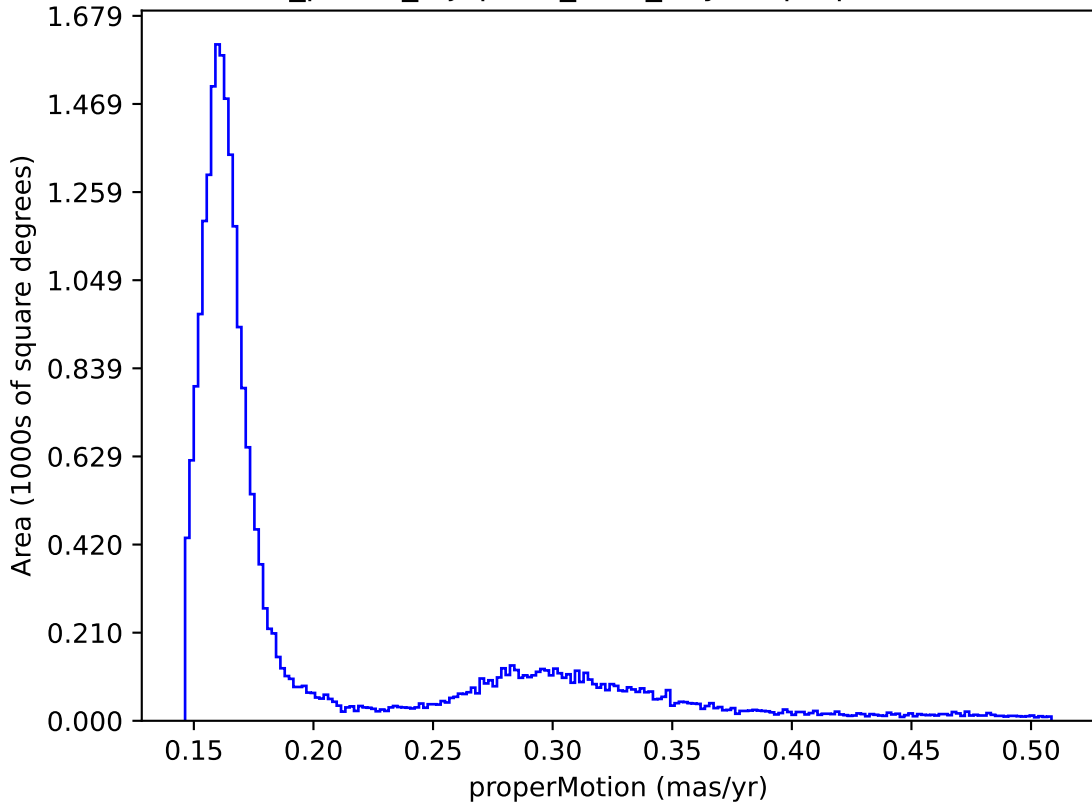
roll_pause_mjdp120_v3.4_10yrs : properMotion
