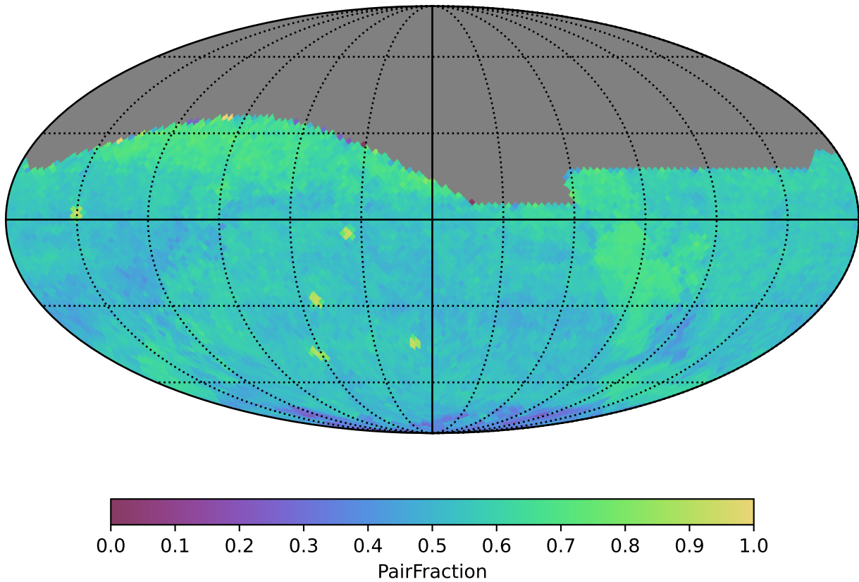
roll_pause_mjdp120_v3.4_10yrs (g or r or i): PairFraction
