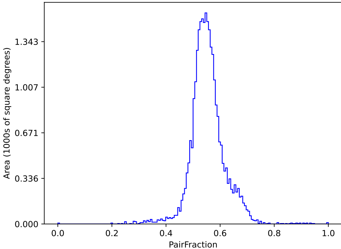
roll_pause_mjdp120_v3.4_10yrs (g or r or i): PairFraction
