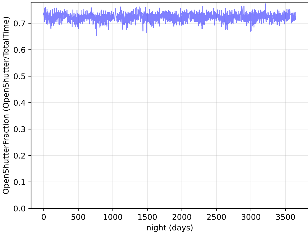
roll_pause_mjdp120_v3.4_10yrs : OpenShutterFraction
