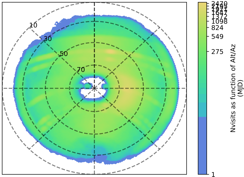
roll_pause_mjdp120_v3.4_10yrs z: Nvisits as function of Alt/Az
