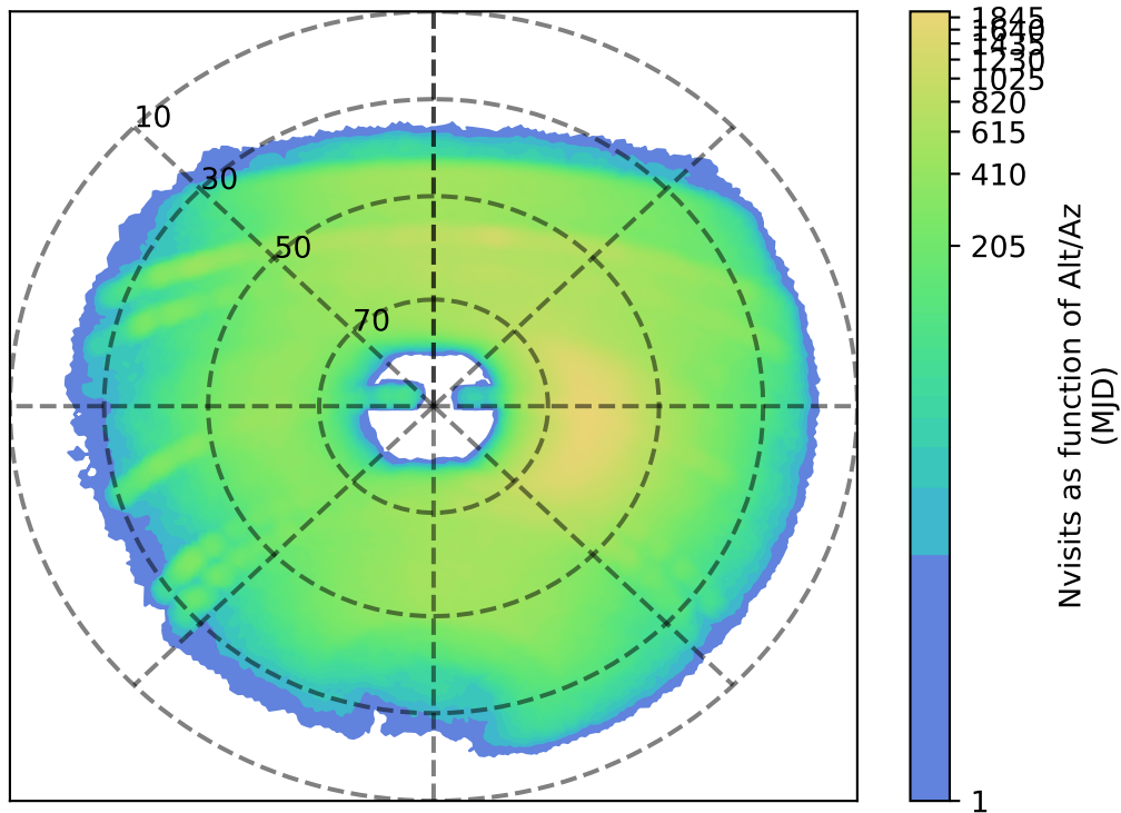
roll_pause_mjdp120_v3.4_10yrs y: Nvisits as function of Alt/Az
