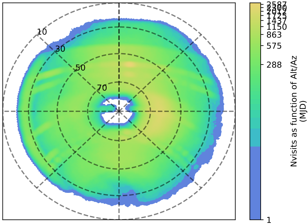
roll_pause_mjdp120_v3.4_10yrs r: Nvisits as function of Alt/Az
