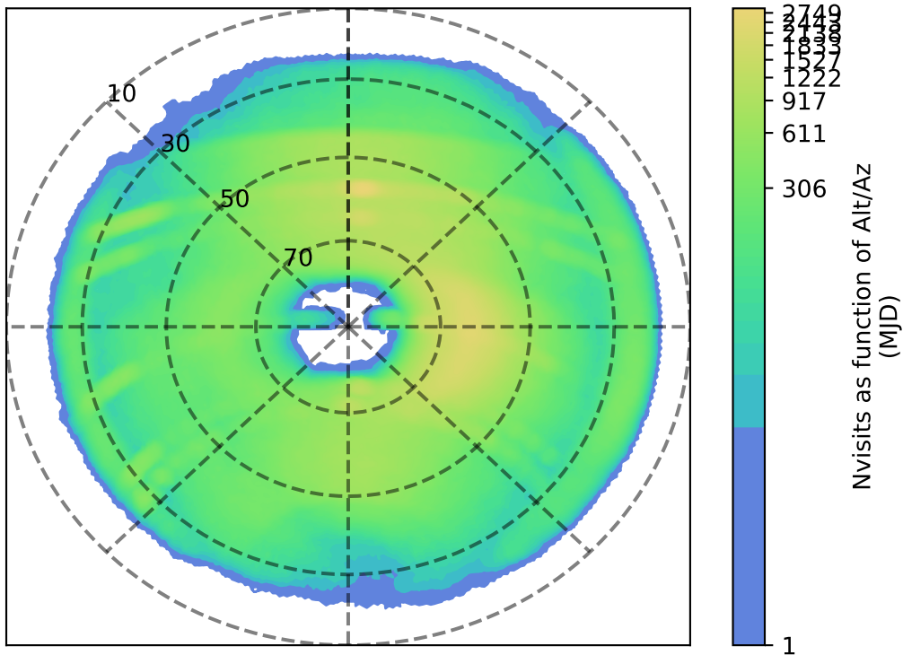
roll_pause_mjdp120_v3.4_10yrs i: Nvisits as function of Alt/Az
