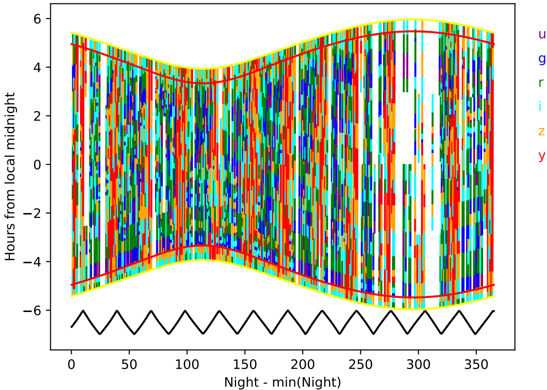
roll_pause_mjdp120_v3.4_10yrs year 8-9: Hourglass
