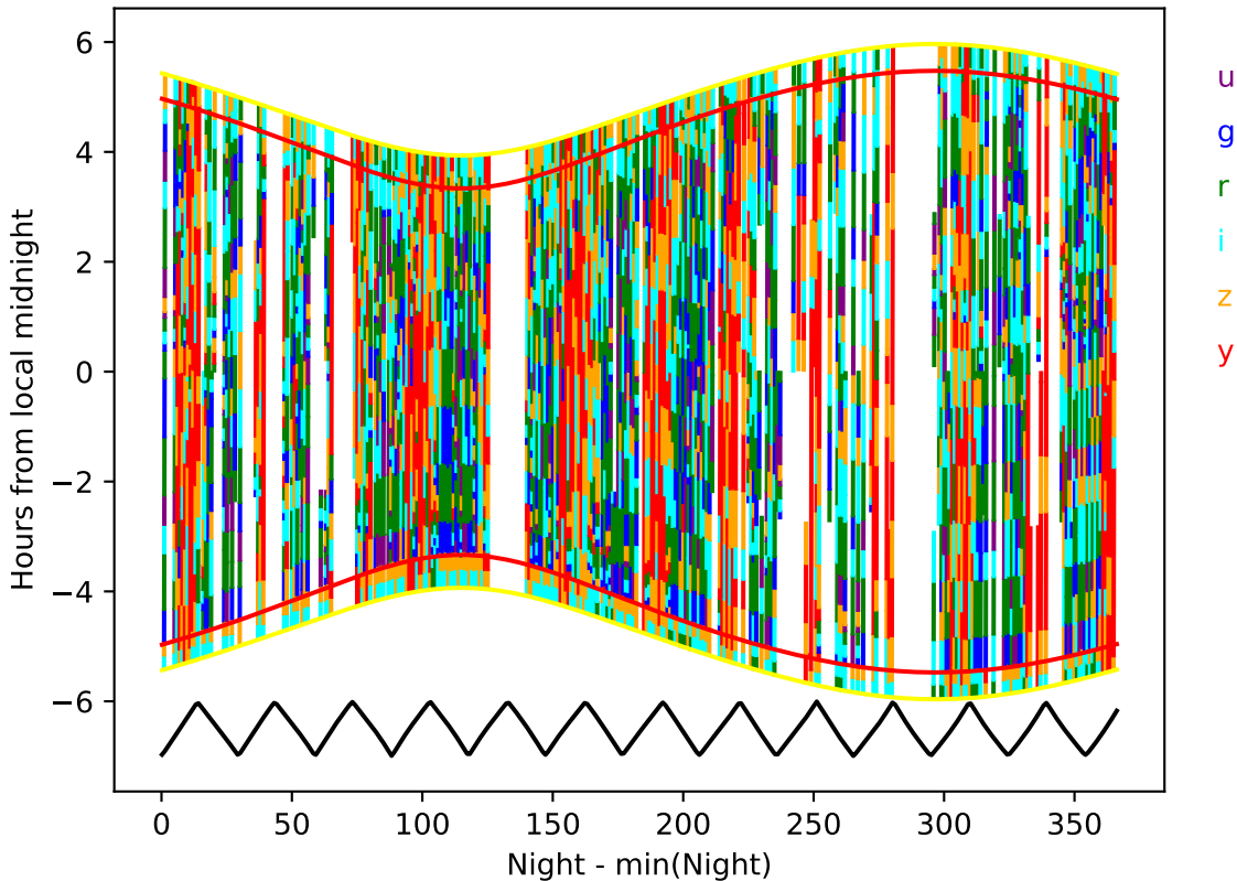
roll_pause_mjdp120_v3.4_10yrs year 5-6: Hourglass
