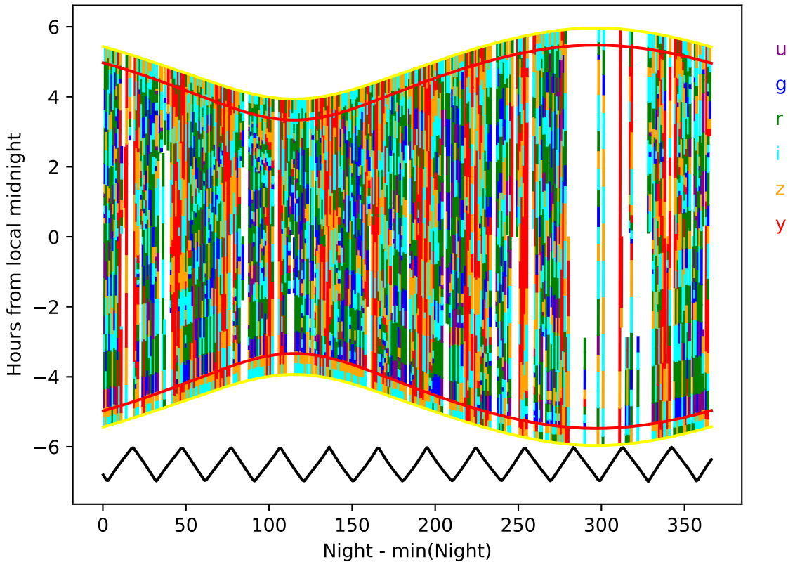
roll_pause_mjdp120_v3.4_10yrs year 2-3: Hourglass
