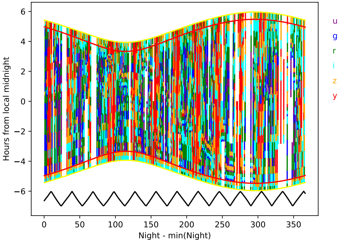
roll_pause_mjdp120_v3.4_10yrs year 0-1: Hourglass
