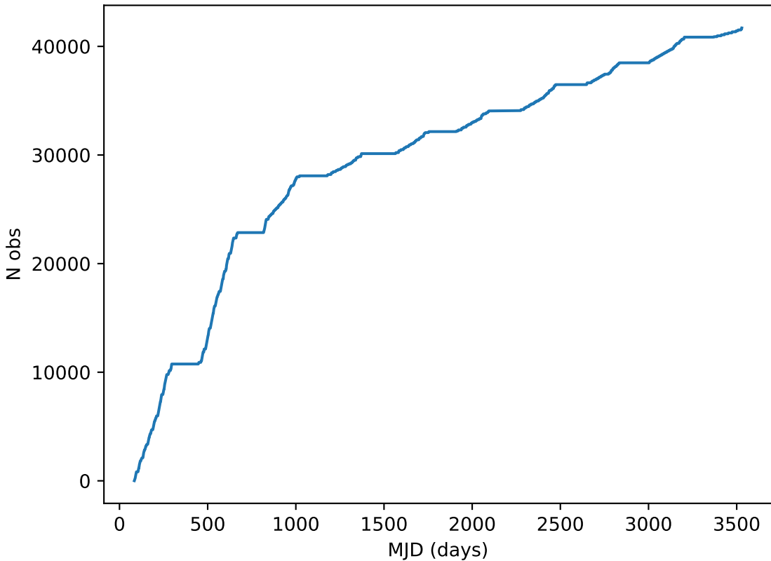
roll_pause_mjdp120_v3.4_10yrs note like DD: COSMOS%: Cumulative
