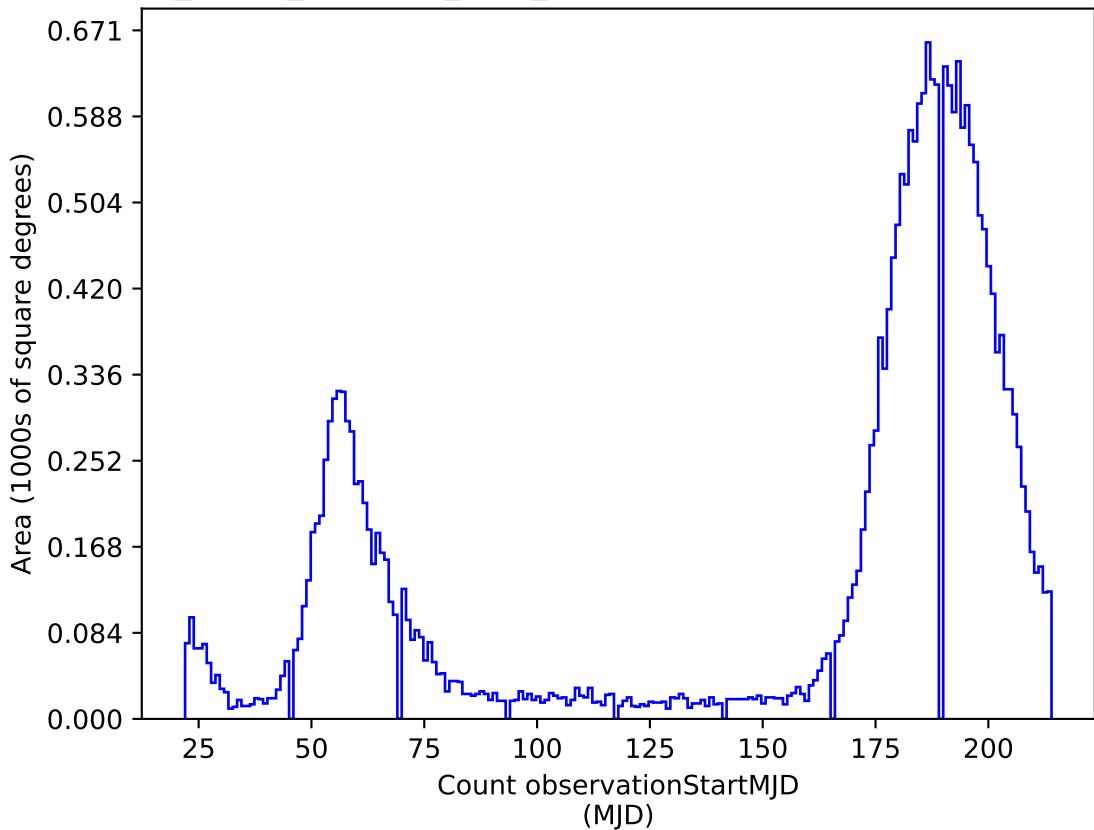
roll_pause_mjdp120_v3.4_10yrs i: Count observationStartMJD
