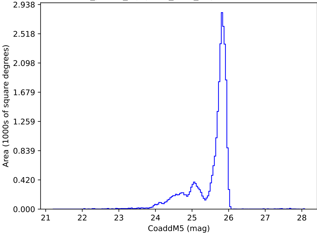
roll_pause_mjdp120_v3.4_10yrs z: CoaddM5
