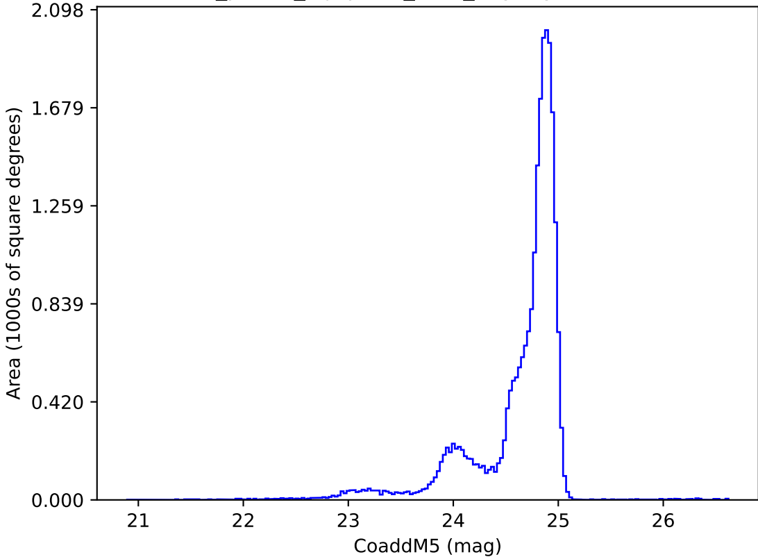
roll_pause_mjdp120_v3.4_10yrs y: CoaddM5
