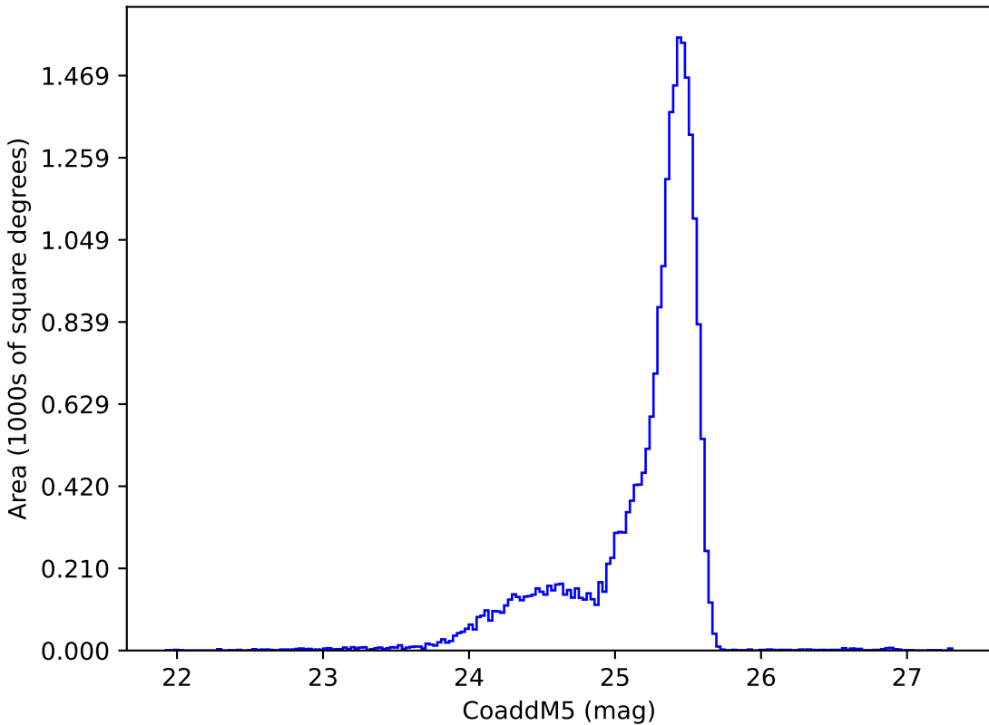
roll_pause_mjdp120_v3.4_10yrs u: CoaddM5
