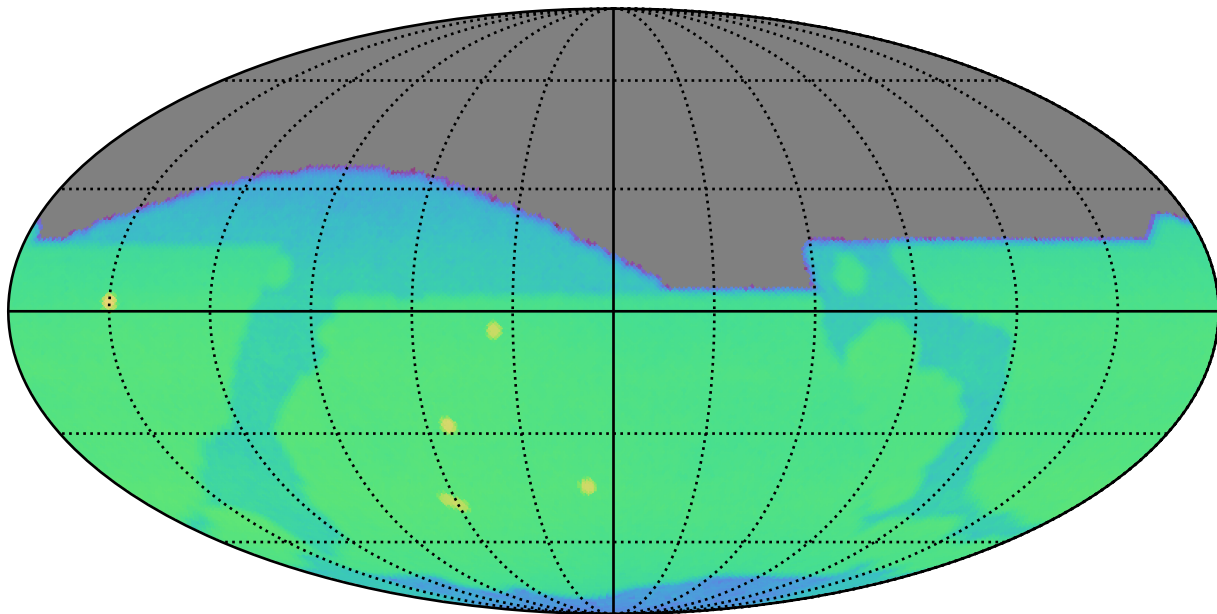
roll_pause_mjdp120_v3.4_10yrs r: CoaddM5
