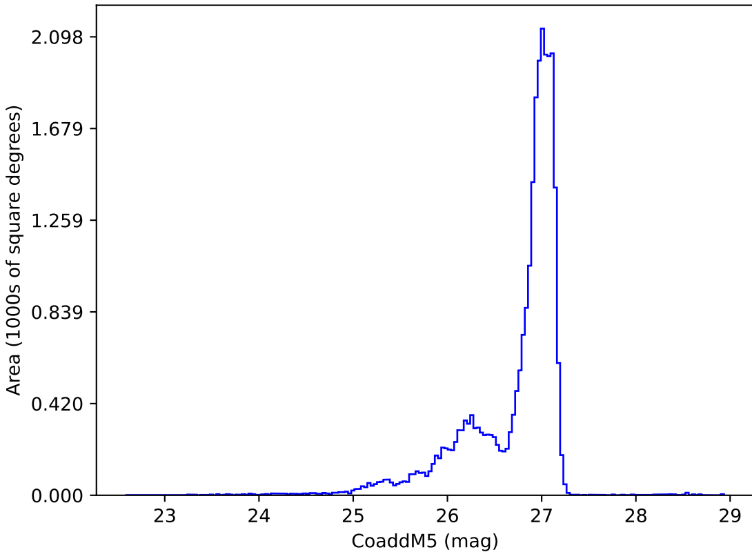
roll_pause_mjdp120_v3.4_10yrs r: CoaddM5
