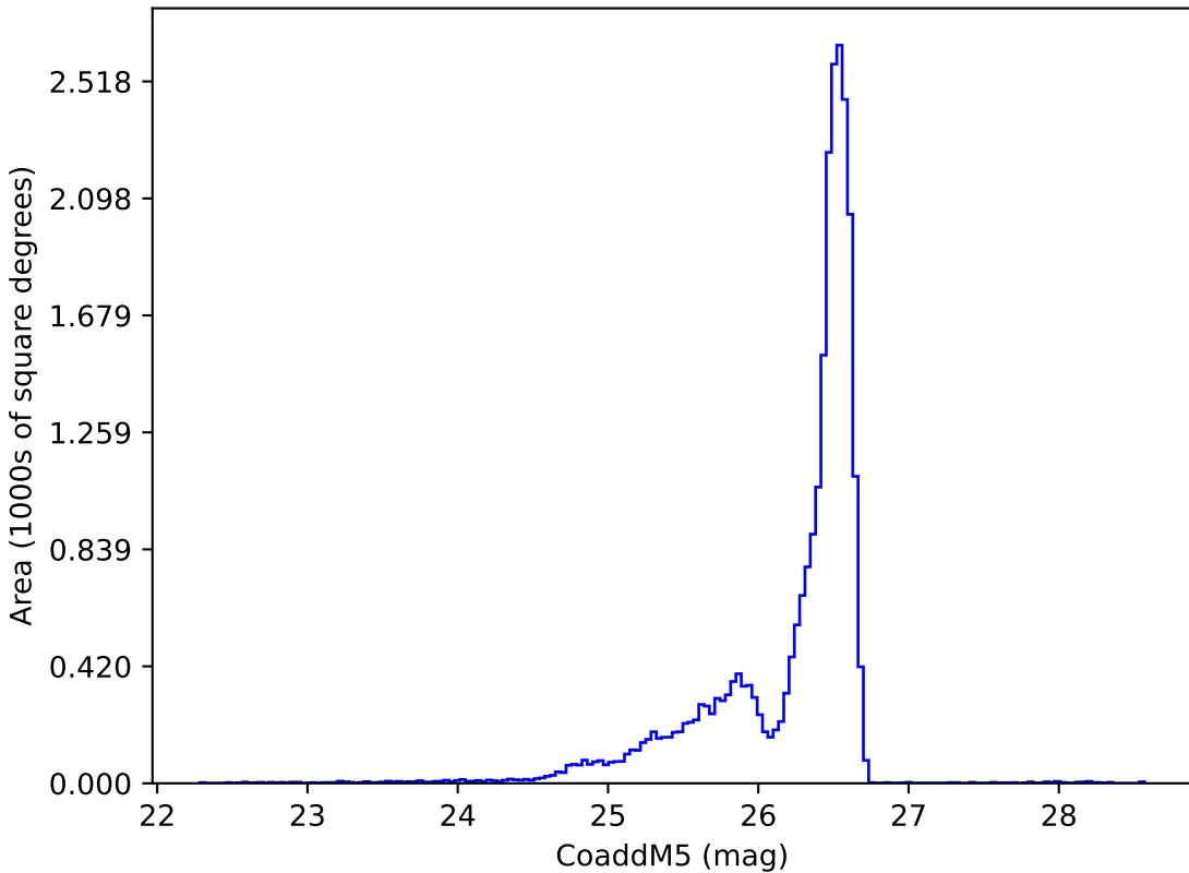
roll_pause_mjdp120_v3.4_10yrs i: CoaddM5
