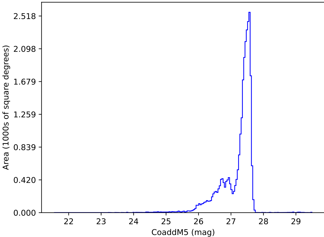
roll_pause_mjdp120_v3.4_10yrs : CoaddM5
