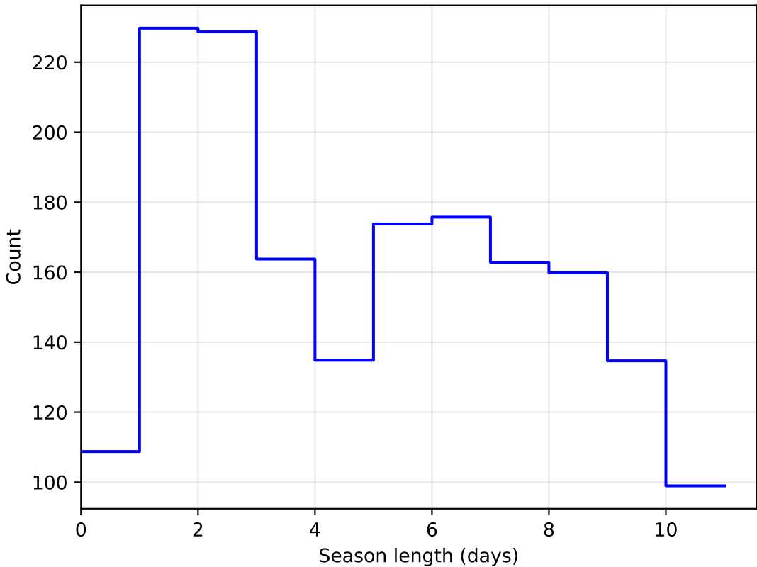
roll_pause_mjdp120_v3.4_10yrs DD:WFD all bands: SeasonLength
