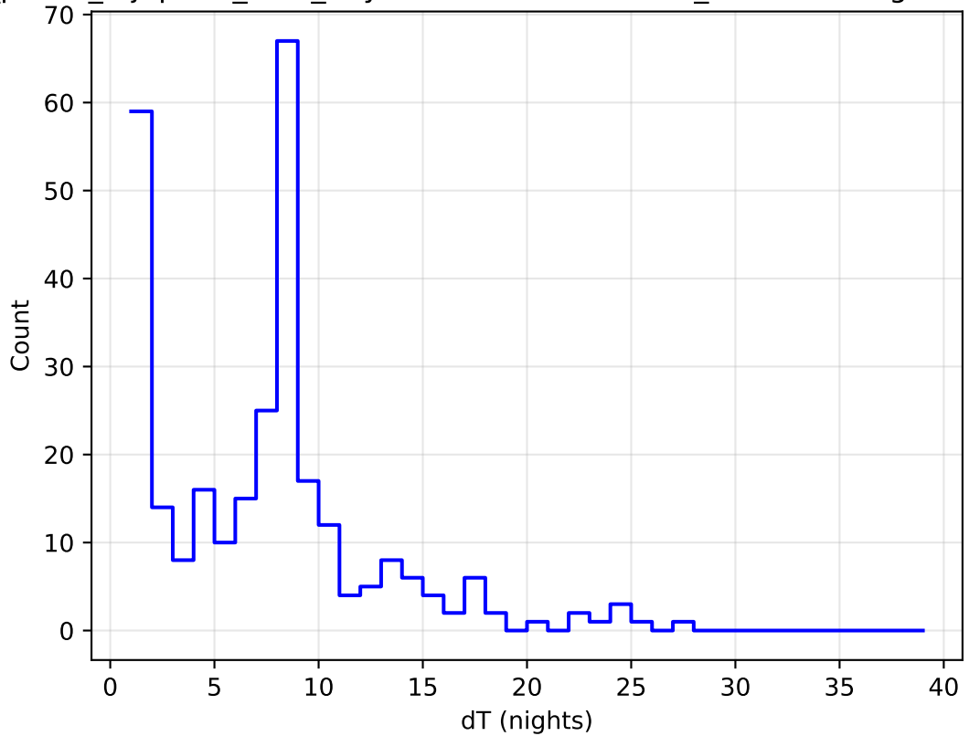
roll_pause_mjdp120_v3.4_10yrs all bands: DD:XMM_LSS Delta Nights Histogram
