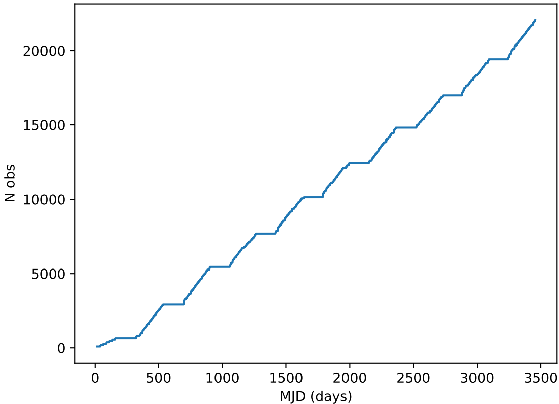
roll_pause_mjdp120_v3.4_10yrs all bands: DD:XMM_LSS Cumulative NVisits
