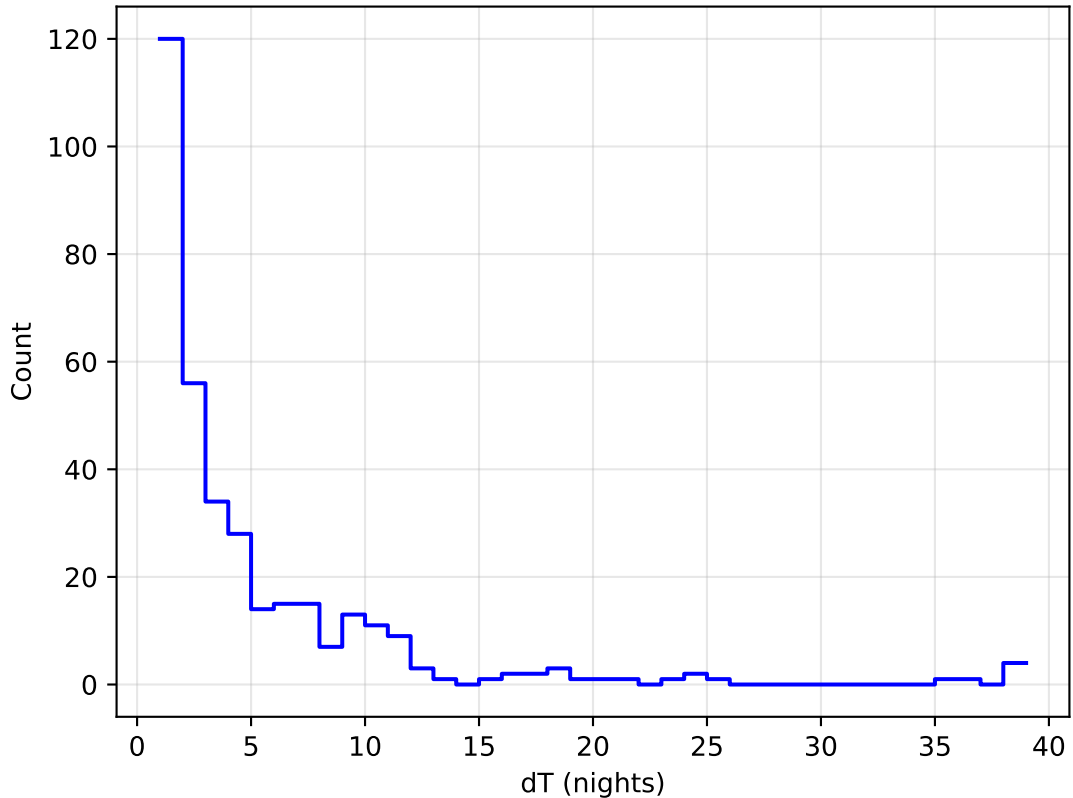
roll_pause_mjdp120_v3.4_10yrs all bands: DD:WFD Delta Nights Histogram
