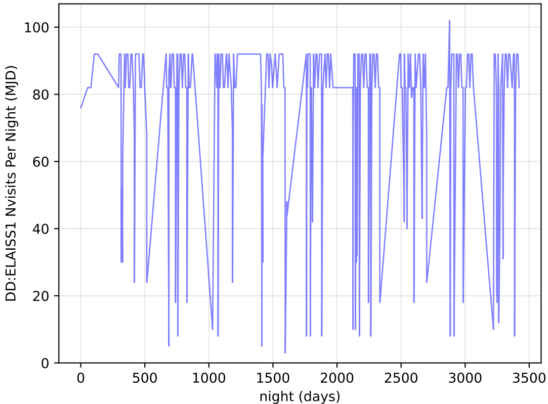
roll_pause_mjdp120_v3.4_10yrs all bands: DD:ELAISS1 Nvisits Per Night
