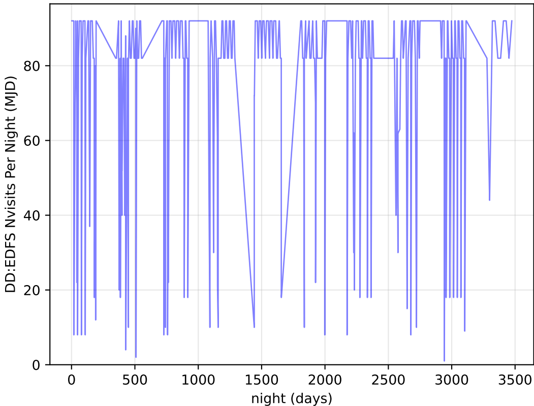
roll_pause_mjdp120_v3.4_10yrs all bands: DD:EDFS Nvisits Per Night
