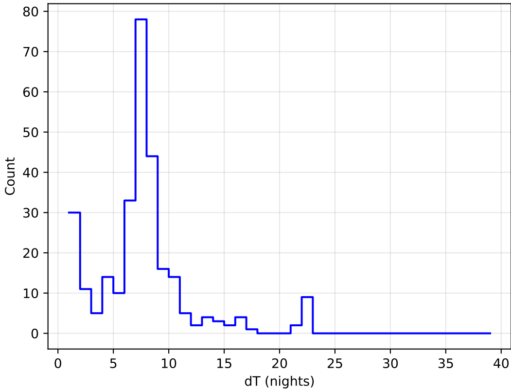
roll_pause_mjdp120_v3.4_10yrs all bands: DD:EDFS Delta Nights Histogram
