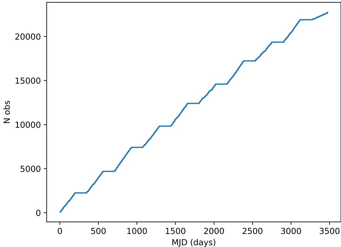
roll_pause_mjdp120_v3.4_10yrs all bands: DD:EDFS Cumulative NVisits
