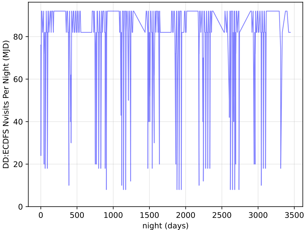
roll_pause_mjdp120_v3.4_10yrs all bands: DD:ECDFS Nvisits Per Night
