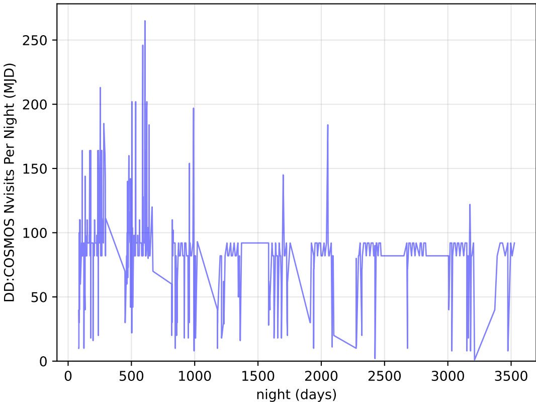
roll_pause_mjdp120_v3.4_10yrs all bands: DD: COSMOS Nvisits Per Night
