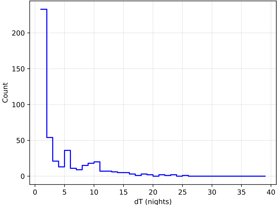
roll_pause_mjdp120_v3.4_10yrs all bands: DD: COSMOS Delta Nights Histogram
