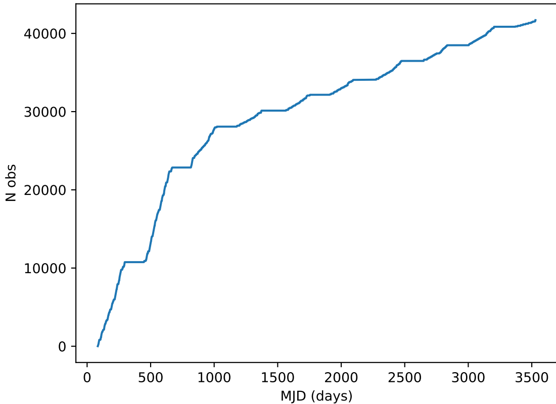
roll_pause_mjdp120_v3.4_10yrs all bands: DD: COSMOS Cumulative NVisits
