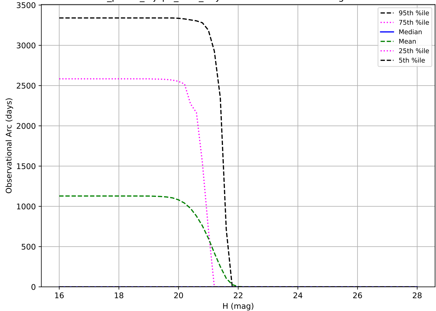
roll_pause_mjdp0_v3.4_10yrs: Observational Arc Length Vatira
