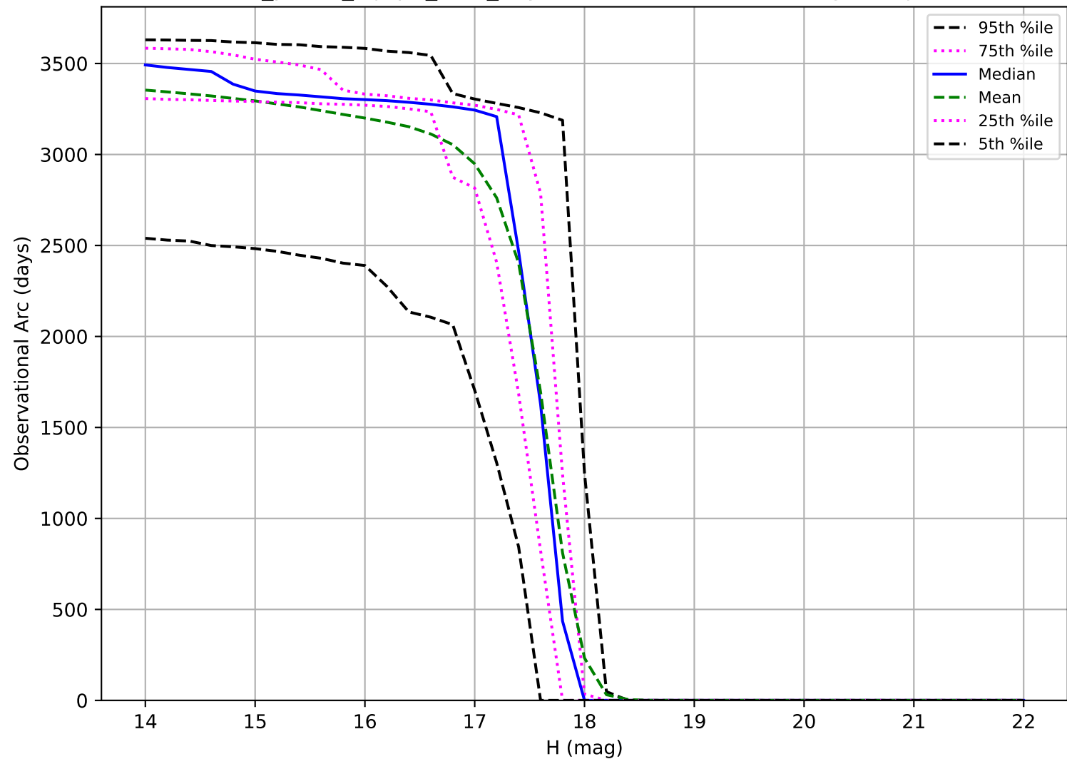
roll_pause_mjdp0_v3.4_10yrs: Observational Arc Length Trojan
