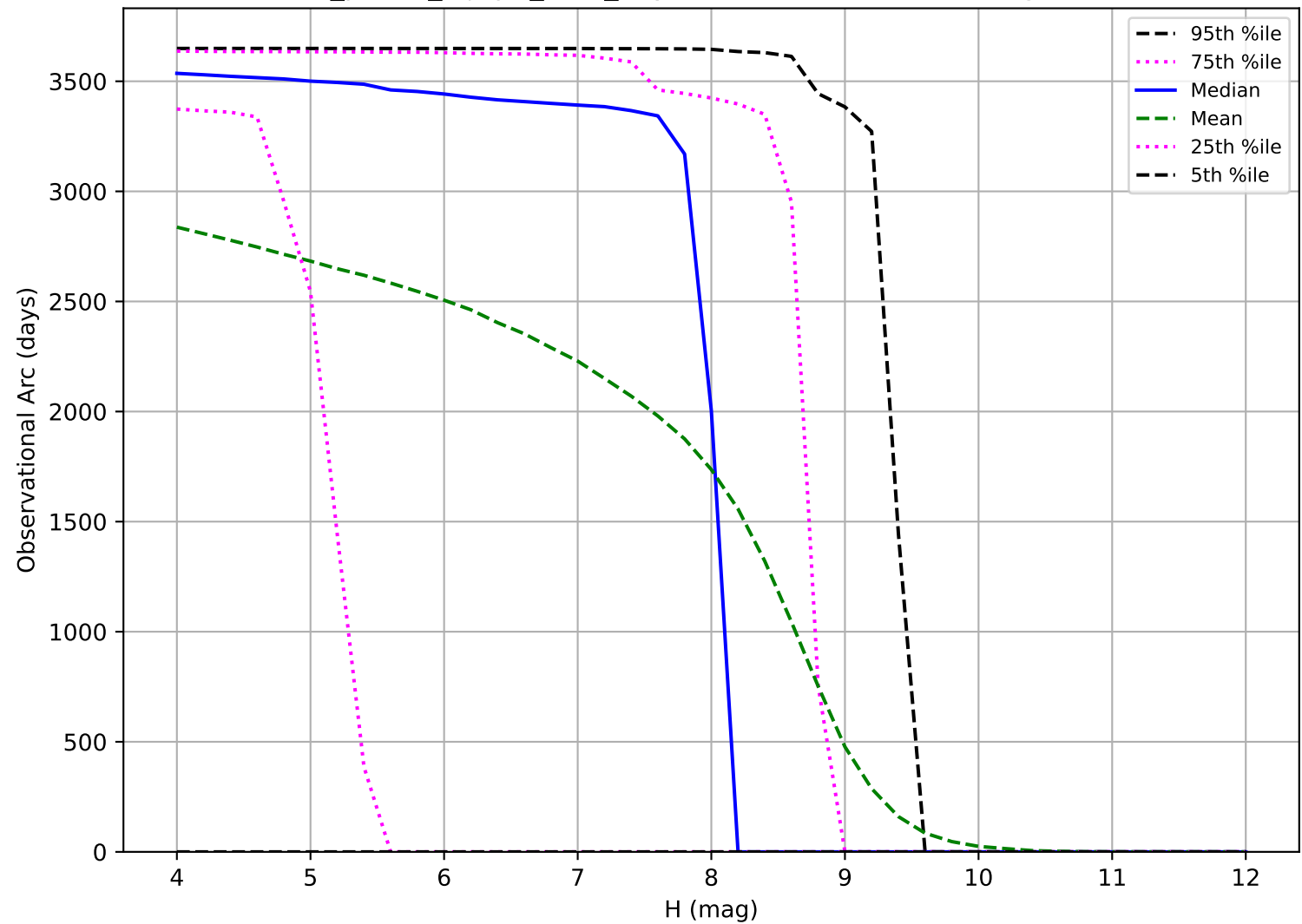
roll_pause_mjdp0_v3.4_10yrs: Observational Arc Length TNO
