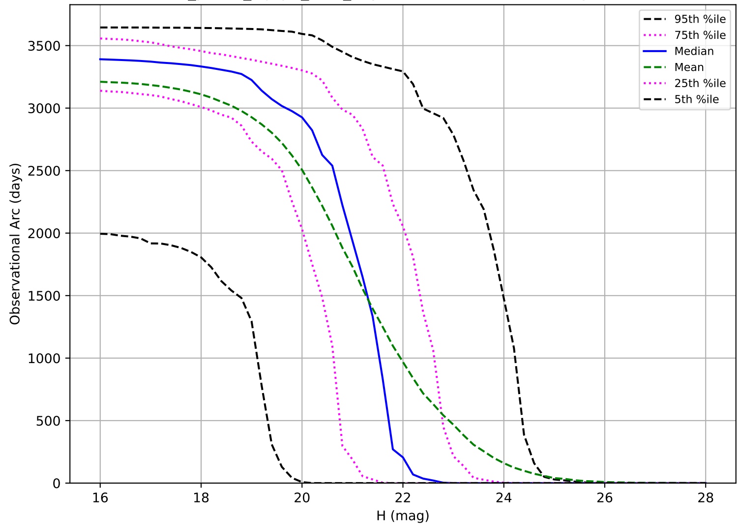
roll_pause_mjdp0_v3.4_10yrs: Observational Arc Length PHA
