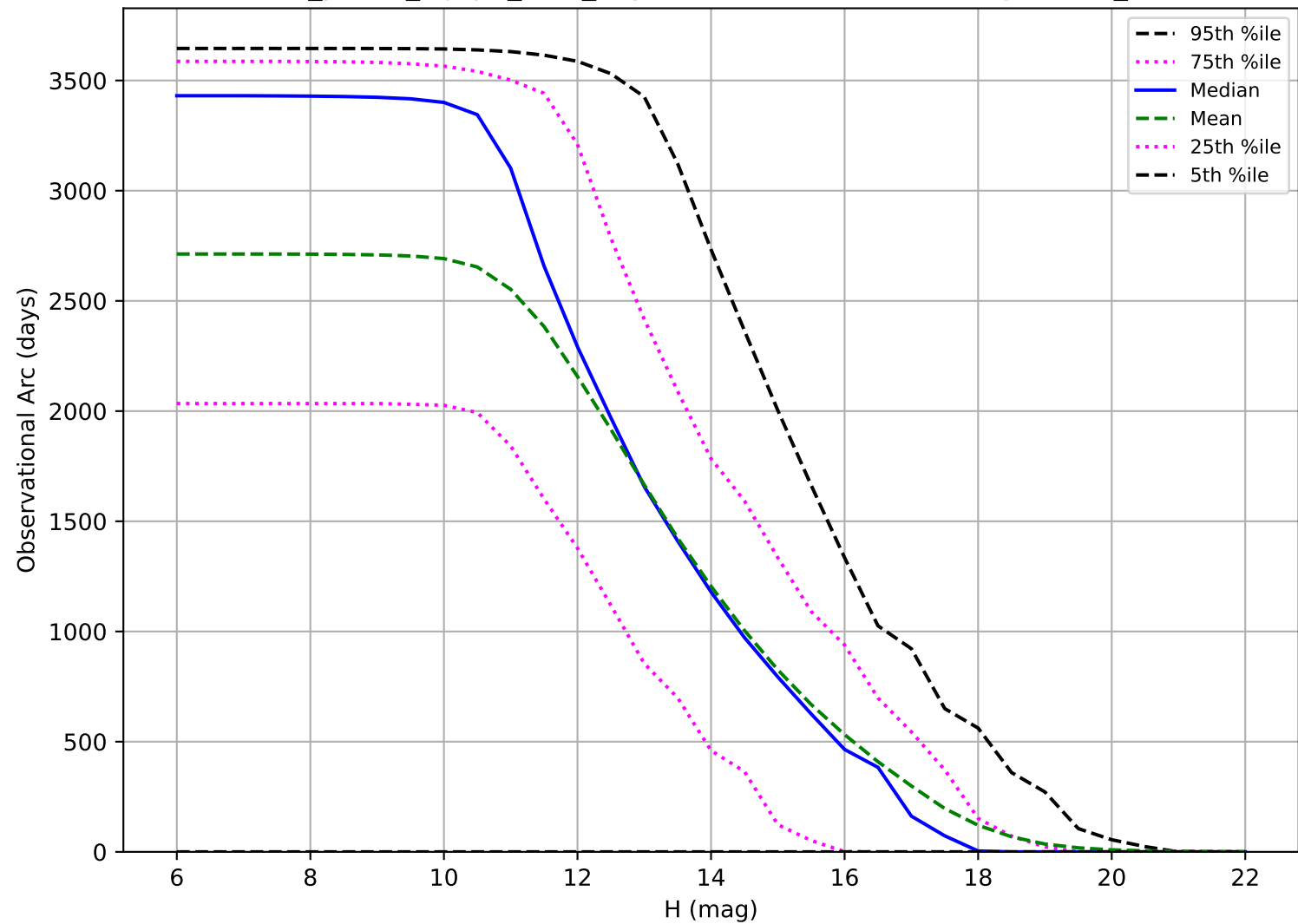
roll_pause_mjdp0_v3.4_10yrs: Observational Arc Length OCC_r5
