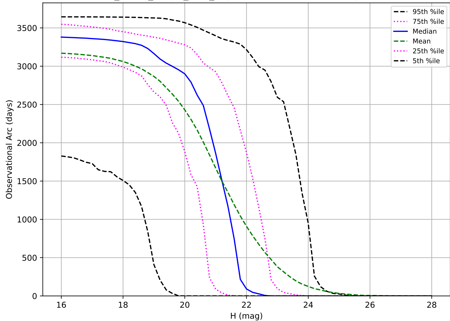
roll_pause_mjdp0_v3.4_10yrs: Observational Arc Length NEO
