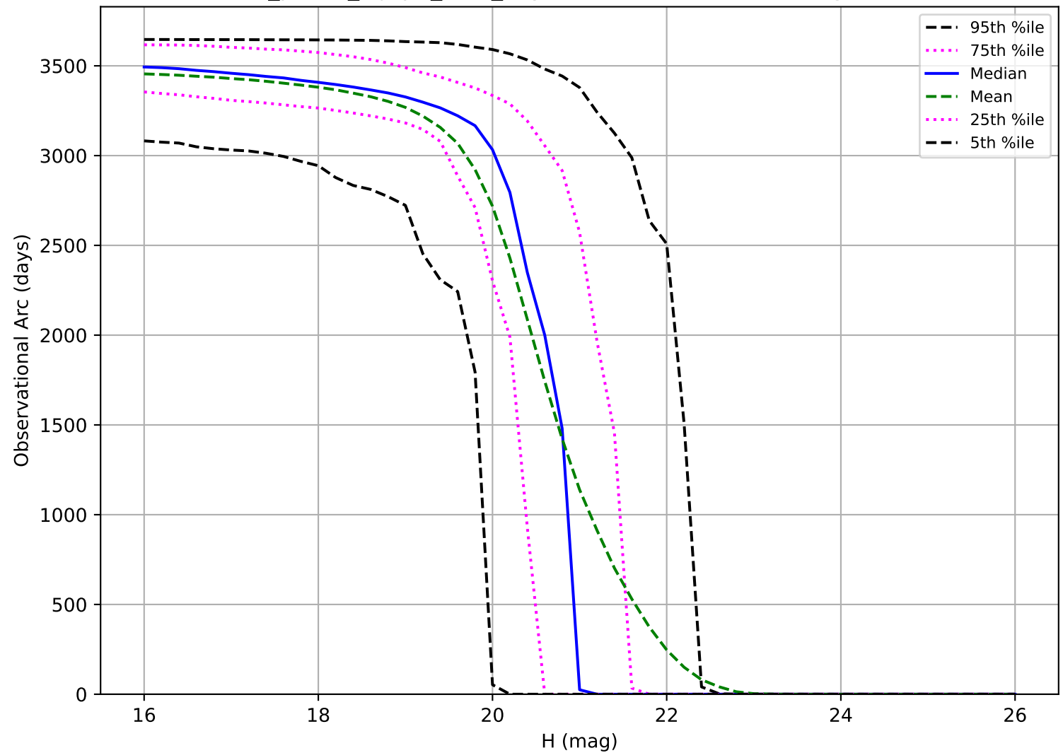
roll_pause_mjdp0_v3.4_10yrs: Observational Arc Length MBA
