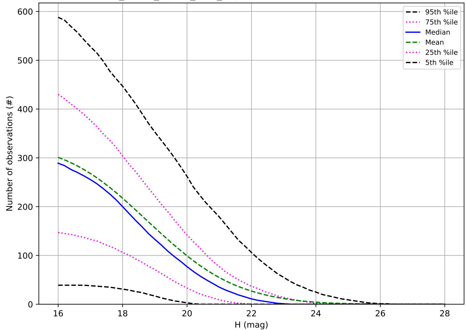
roll_pause_mjdp0_v3.4_10yrs: Number of observations PHA
