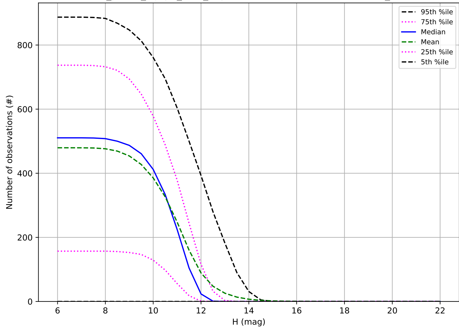
roll_pause_mjdp0_v3.4_10yrs: Number of observations OCC_r20
