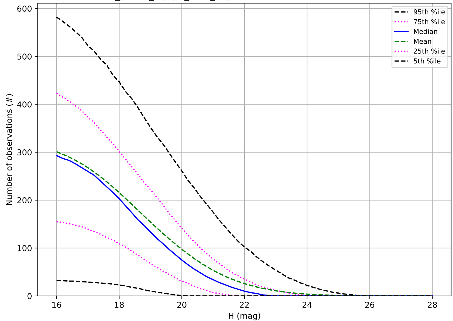
roll_pause_mjdp0_v3.4_10yrs: Number of observations NEO
