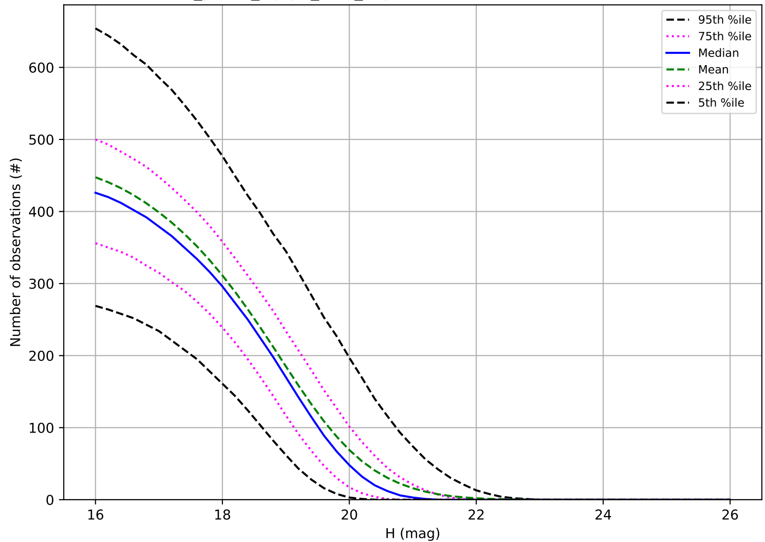
roll_pause_mjdp0_v3.4_10yrs: Number of observations MBA
