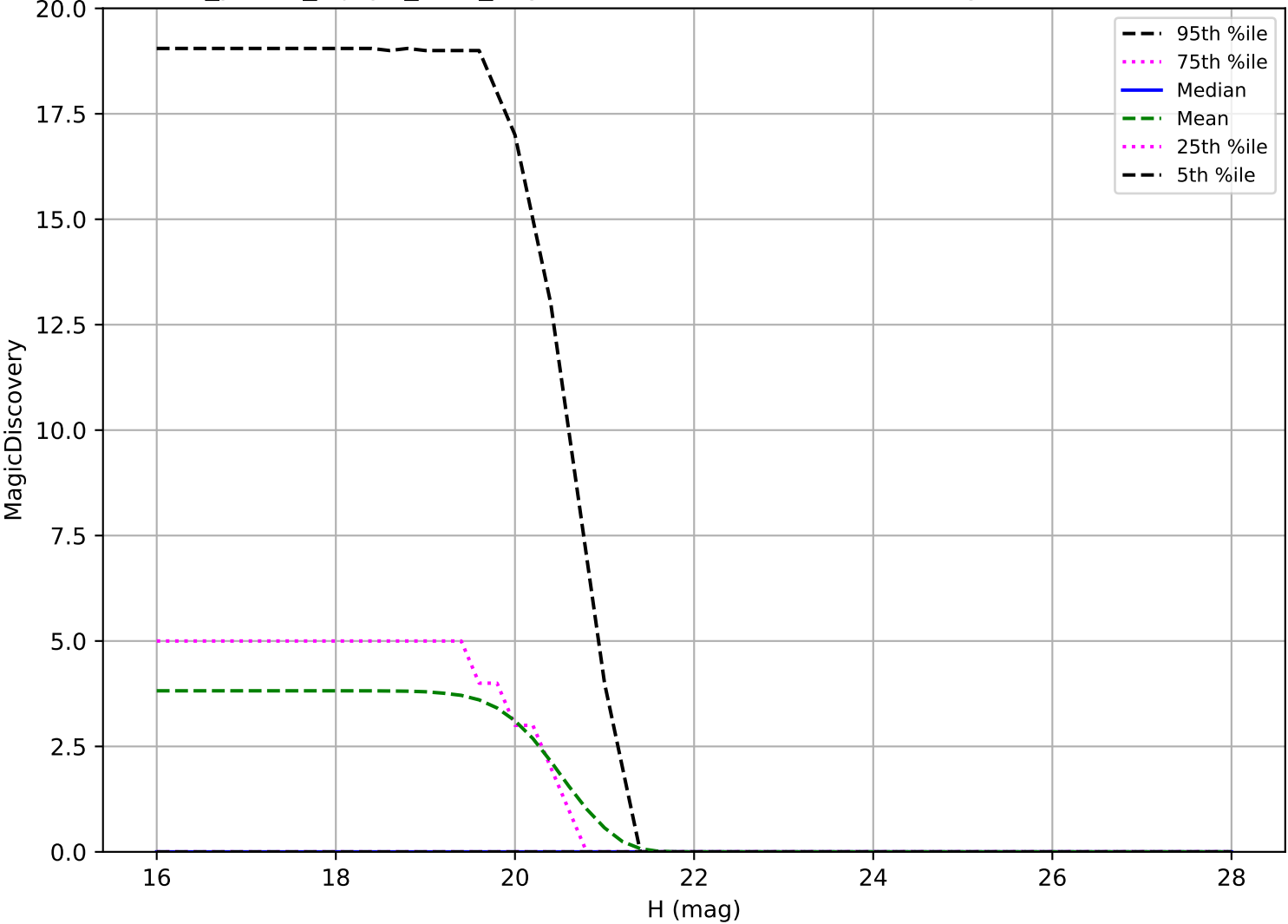
roll_pause_mjdp0_v3.4_10yrs: Vatira 6 detections in 60 nights detection loss
