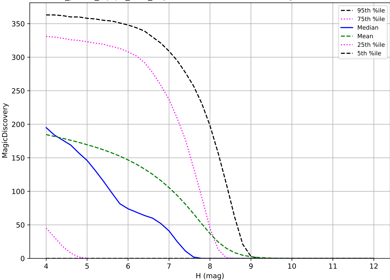
roll_pause_mjdp0_v3.4_10yrs: TNO 6 detections in 60 nights detection loss
