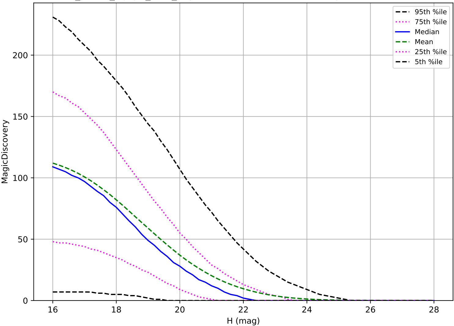
roll_pause_mjdp0_v3.4_10yrs: PHA 6 detections in 60 nights detection loss
